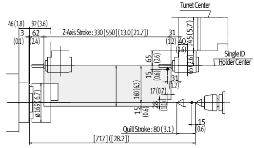
Angular Rev. Tool Head
