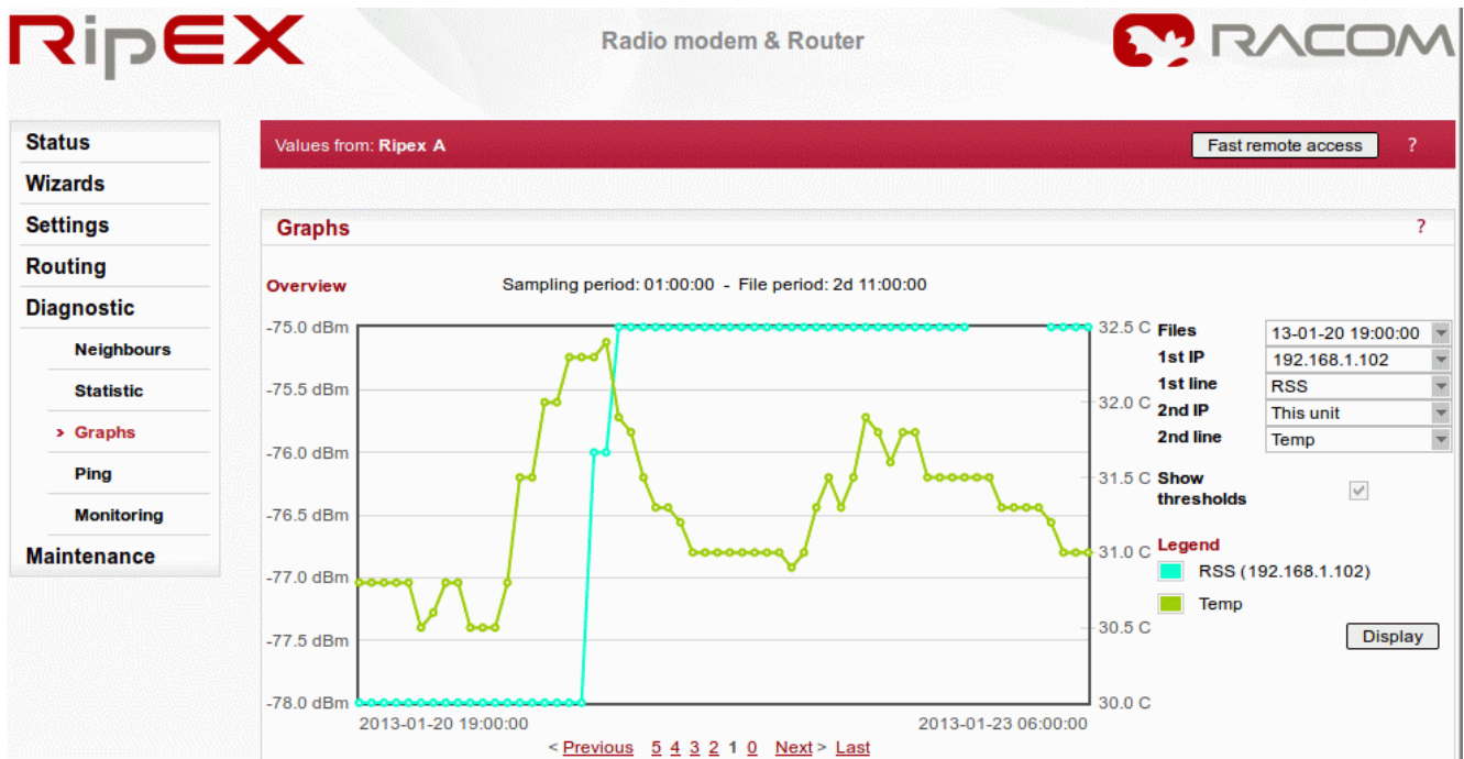
Fig. 3.27: Graph menu
