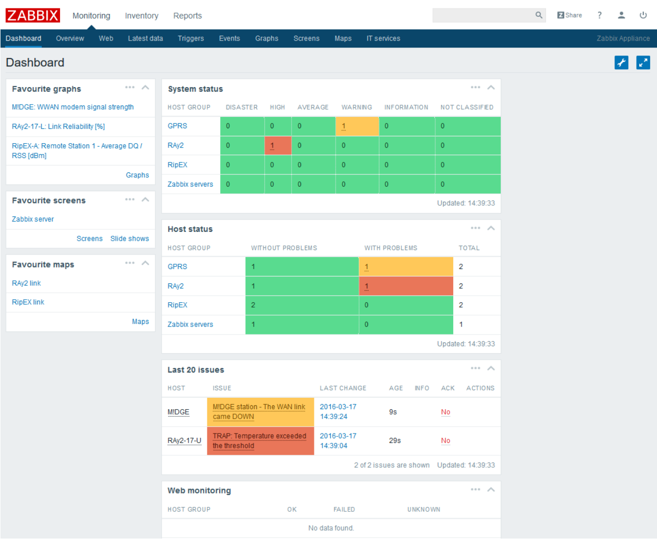
Fig. 2.2: Dashboard
