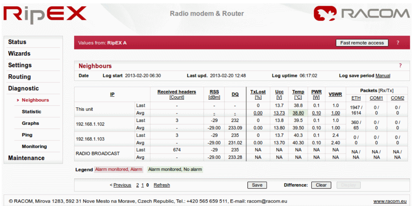
Fig. 3.25: Neighbours menu
