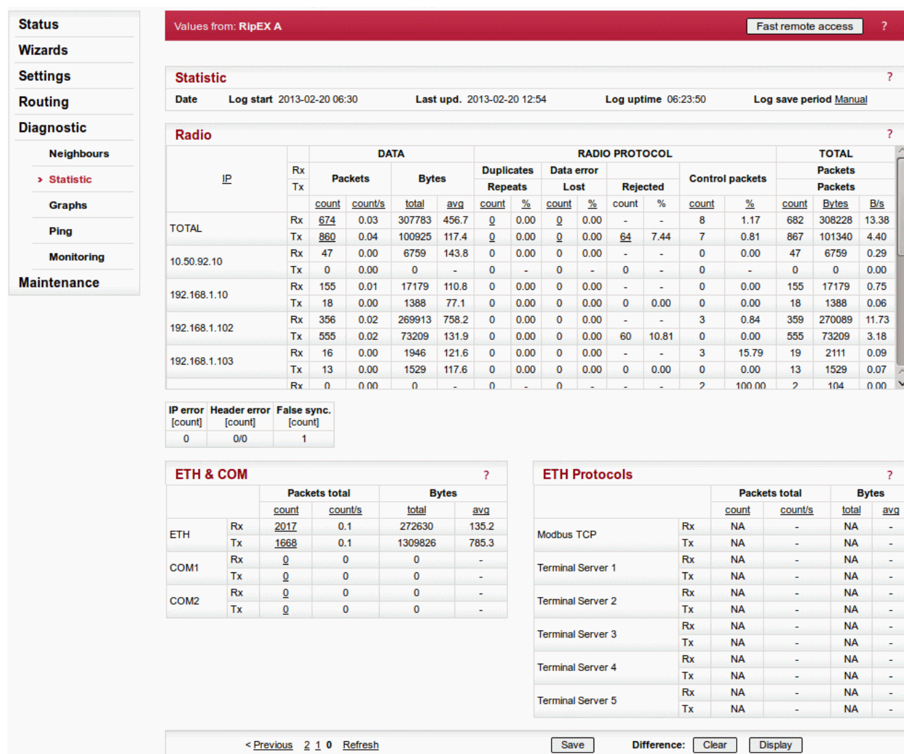
Fig. 3.26: Statistic menu
