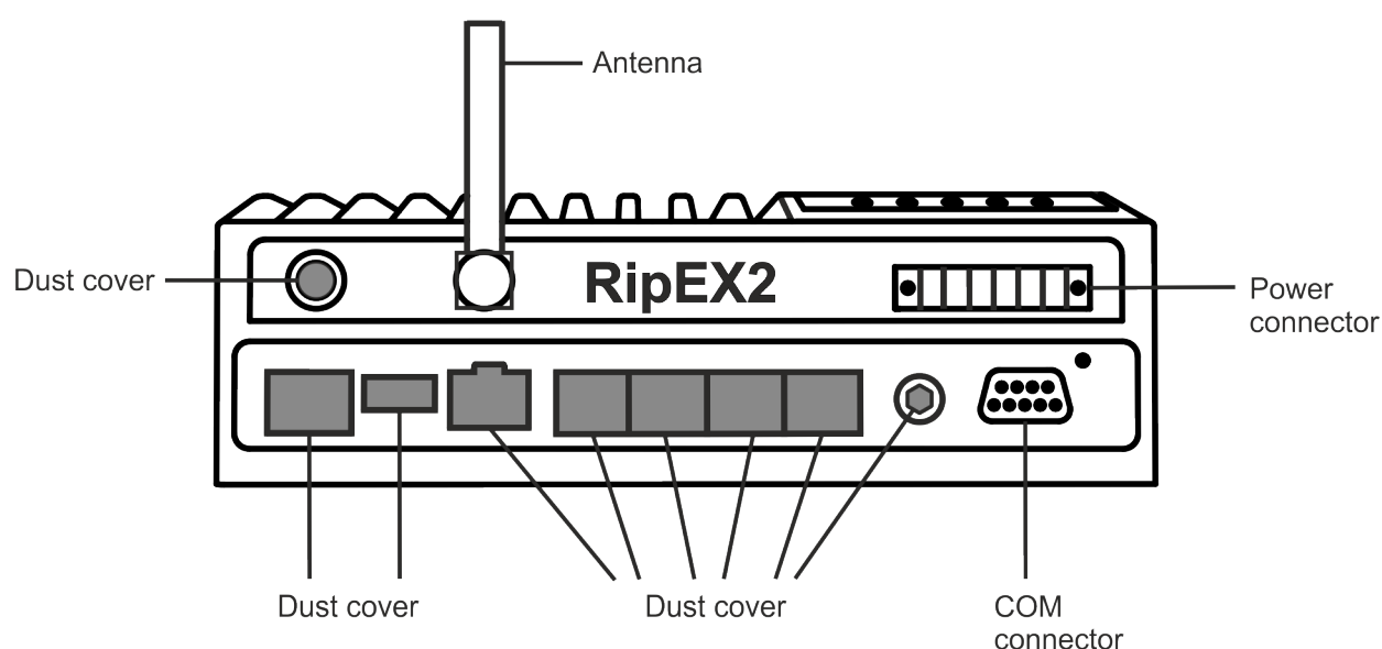
Fig. 4.8: IP5x protection
