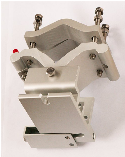
Fig. 5.22: Arkivator antenna bracket (2012) Fig. 5.23: Bracket on the mast, version 2012
