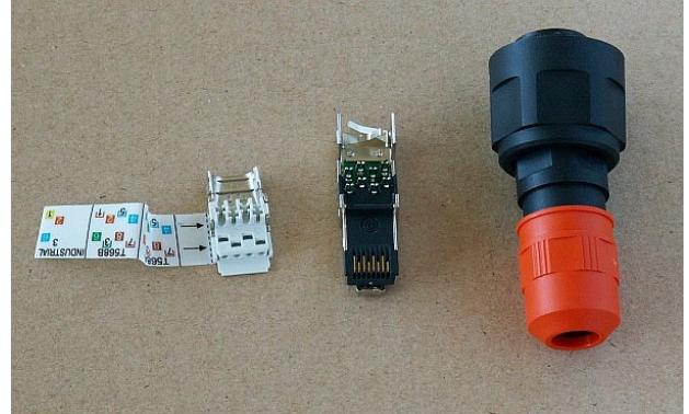
Fig. 5.32: IE-PI-RJ45-FH connector before fitting
