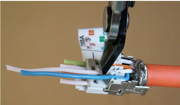
Fig. 5.41: Cutting off of the upper conductors
