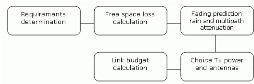
Fig. 2.7: Design flowchart
