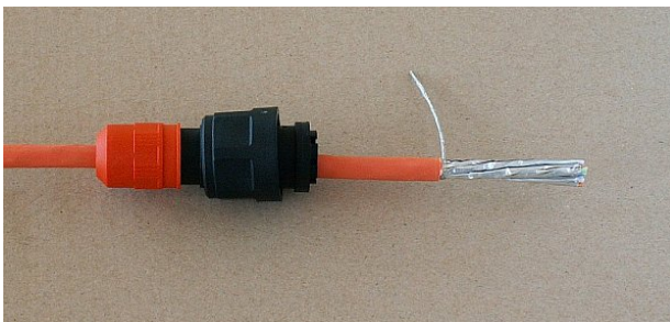
Fig. 5.35: Twisted shielding
