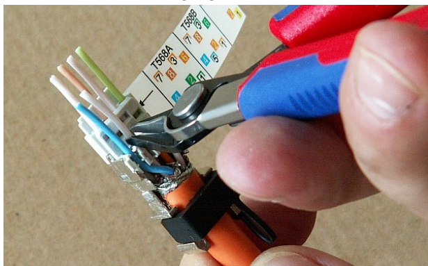
Fig. 5.57: Trimming conductors
