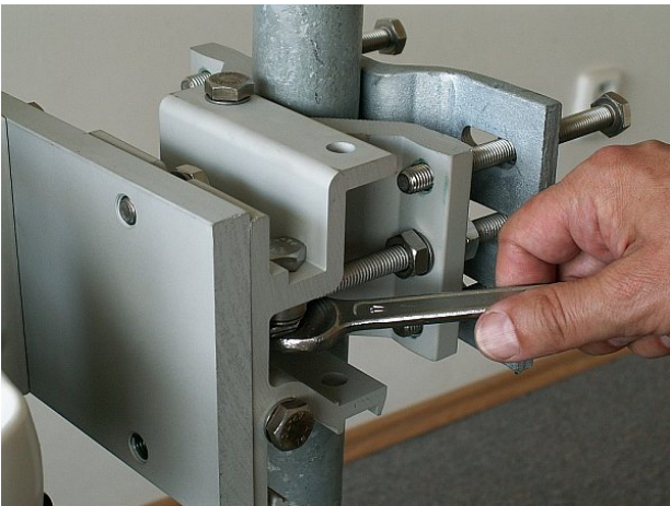
Fig. 5.18: Tightening the axis at the fine adjustment bolt
