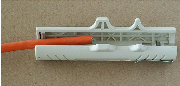
Fig. 5.49: Removing insulation
