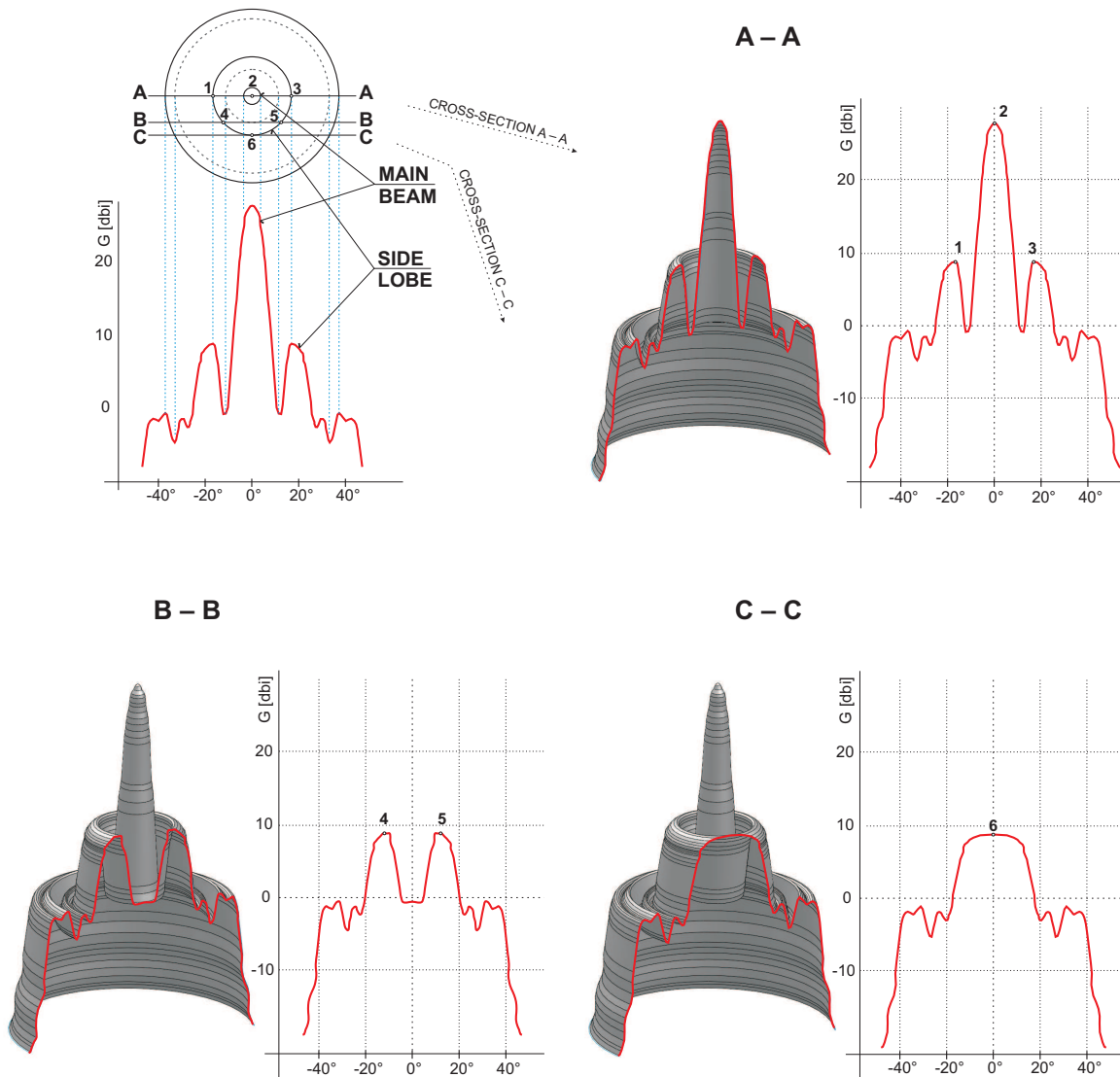
Fig. 5.71: Radiation diagrams
