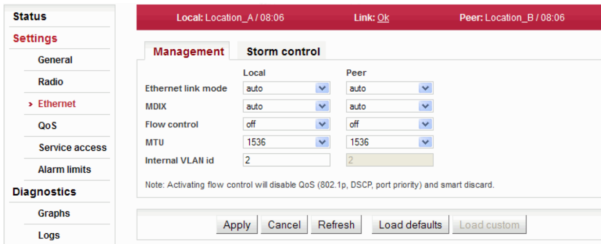
Fig. 6.8: Configuration menu Settings – Ethernet
