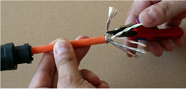
Fig. 5.37: Trimming shielding
