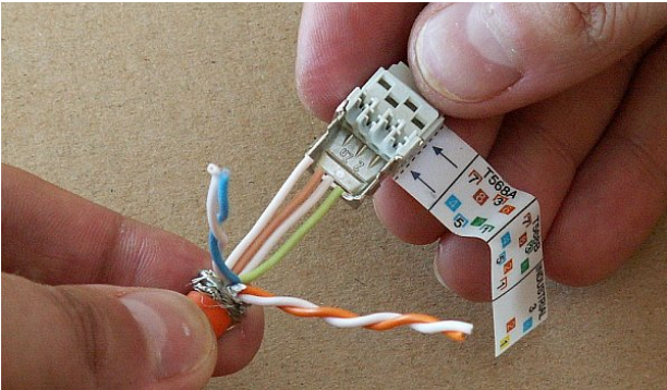
Fig. 5.39: Pushing the lower pairs into the connector
