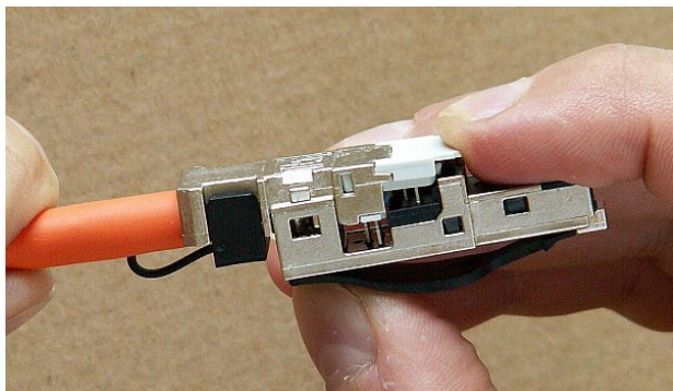
Fig. 5.59: Fitting the mate to the internal connector
