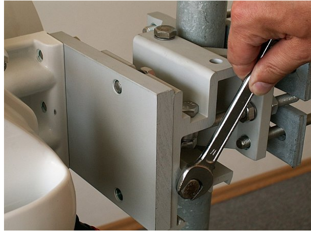
Fig. 5.17: Vertical adjustment of the antenna direction
