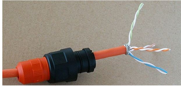
Fig. 5.38: Separated pairs of conductors
