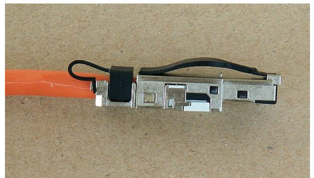
Fig. 5.48: Finished connector IE-PS-RJ45-FH-BK
