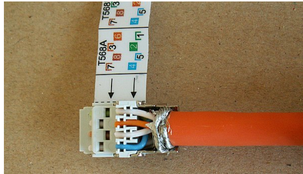
Fig. 5.42: All conductors in the connector
