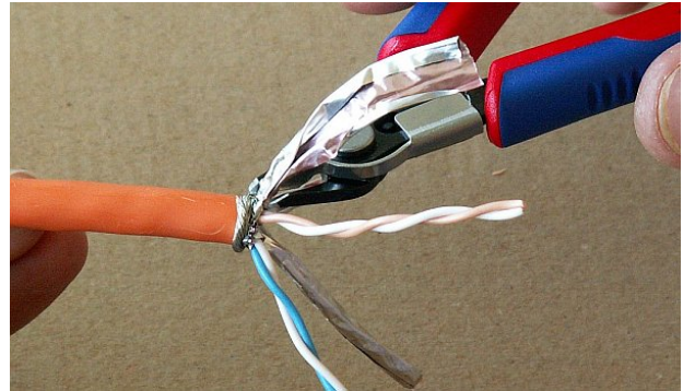
Fig. 5.52: Removing aluminium conductor shielding
