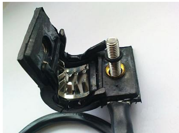
Fig. 5.64: Grounding kit detail
