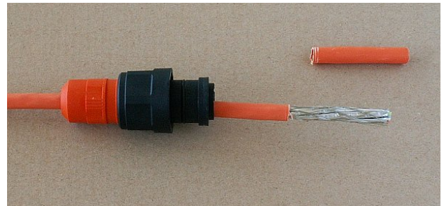
Fig. 5.34: Insulation removed
