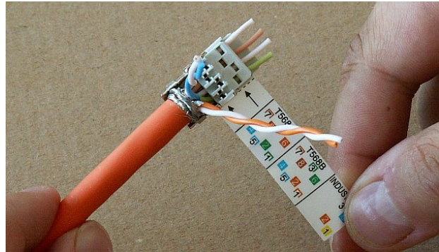
Fig. 5.40: Lower pairs pushed in
