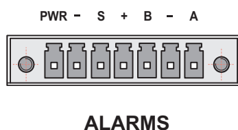
Fig. 3.10: Alarm connector
