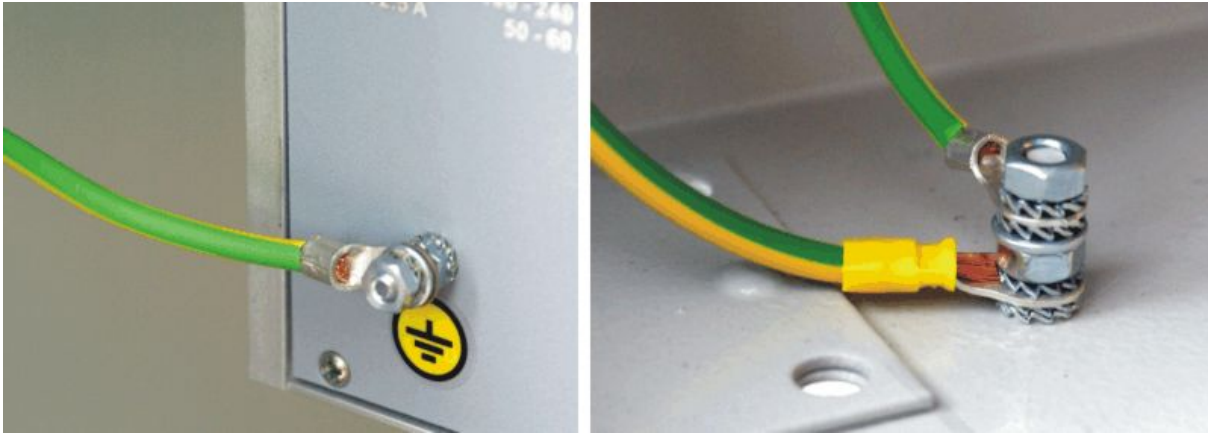
Fig. 4.5: RipEX-HS grounding in a cabinet
