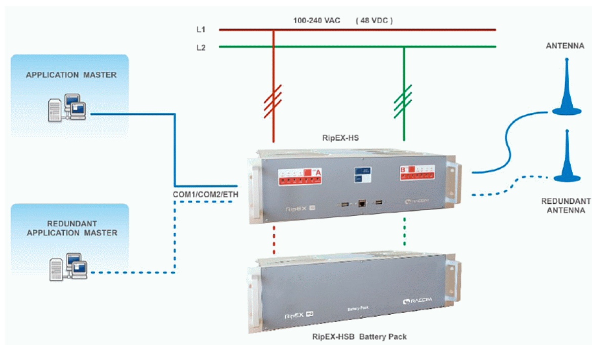
Fig. 4.1: HS connected as a SCADA centre redundant radio modem
