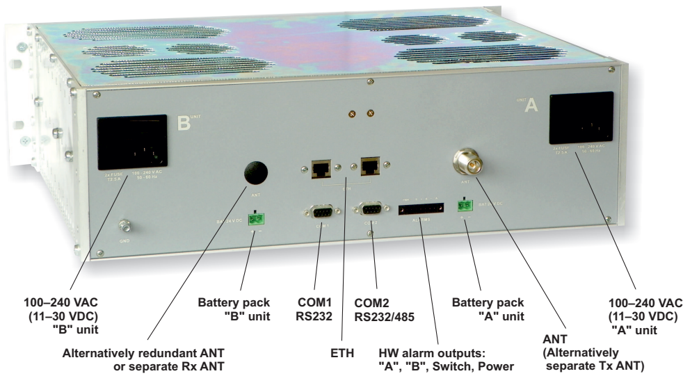
Fig. 3.6: RipEX-HS rear panel
