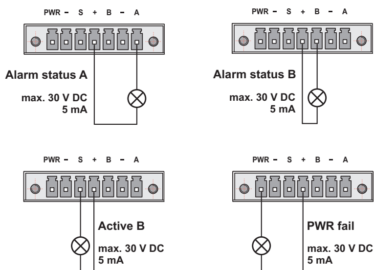
Fig. 3.12: Alarms Outputs
