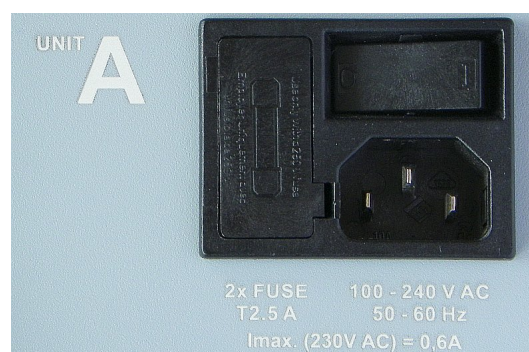
Fig. 3.13: Power supply connector AC model
