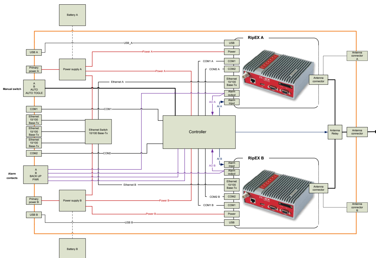
Fig. 2.1: Block diagram
