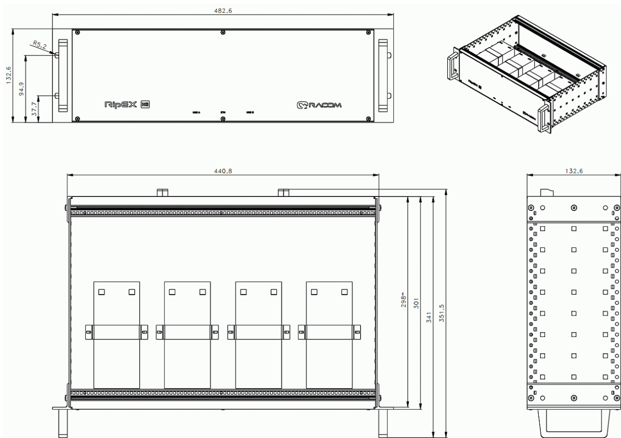
Fig. 3.18: RipEX-HSB dimensions [mm]
