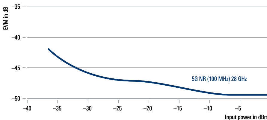
Residual EVM over signal power for a 100 MHz wide 5G NR uplink signal at 28 GHz
